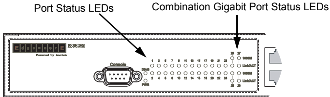
Figure 1-3. ES3528M Port Status LEDs
