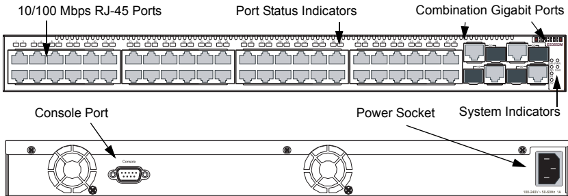
Figure 1-2. ES3552M Front and Rear Panels
