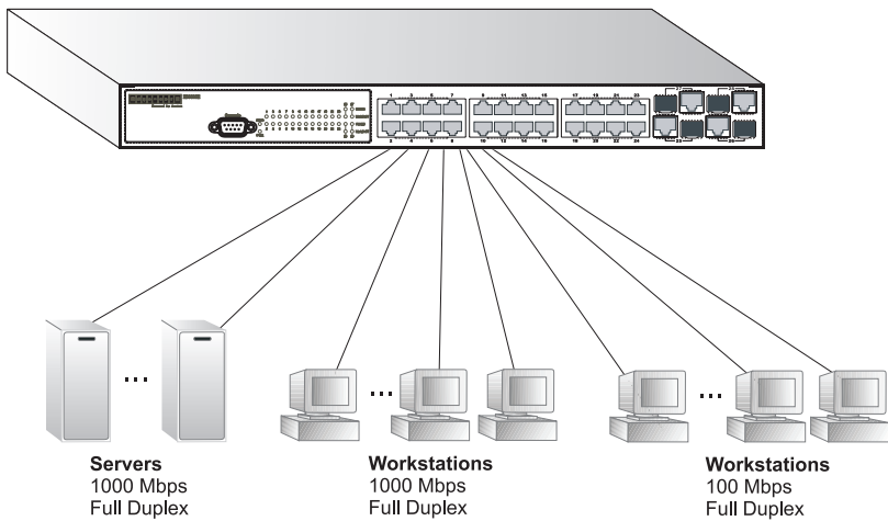
Figure 2-1. Collapsed Backbone
