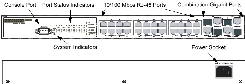
Figure 1-1. ES3528M Front and Rear Panels
