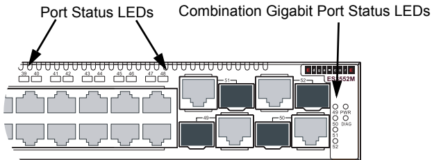
Figure 1-4. ES3552M Port Status LEDs
